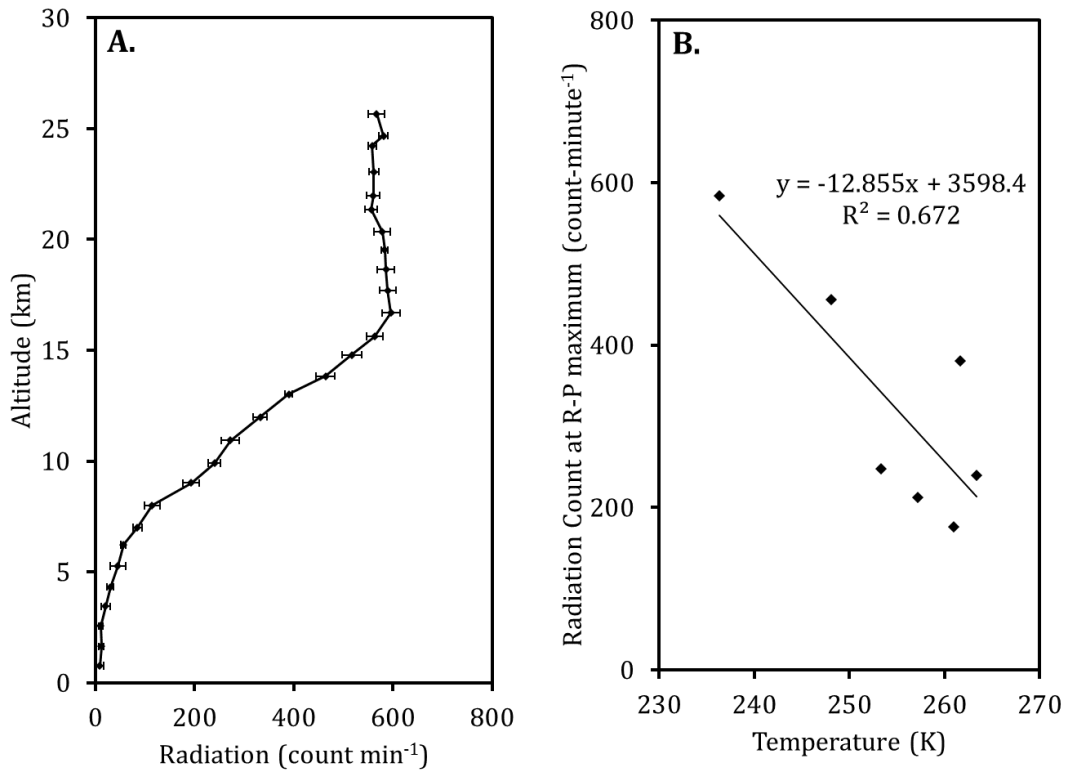
Fig. 2 (A.) Radiation profile measured by on-board Geiger counter. (B.) relationship of Regener-Pfotzer (R-P) maximum with temperature
