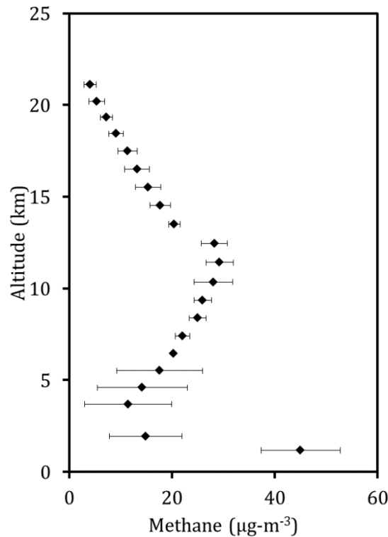
Fig. 2 Methane profile measured with balloon borne MQ-2 detector. The MQ-6 sensor did not measure any changes in concentration.
