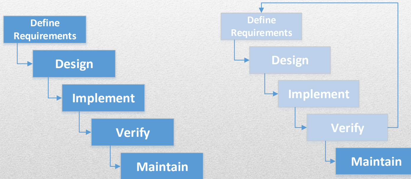
Figure 1. (a) Waterfall model of software development (left, simplified from [35]), (b) Adapted iterative waterfall model of software development (right).
