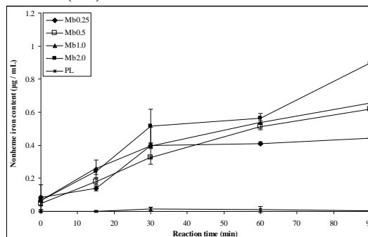
Figure 2. Formation of nonheme iron in a phospholipid liposome model system with various concentrations of metMb during incubation at 37 °C for 90 min (µg nonheme iron/mL metMb-liposome solution). The concentrations of metMb in 50 mM acetate buffer (pH 5.6) were 2 (Mb2.0), 1 (Mb1.0), 0.5 (Mb0.5), and 0.25 (Mb0.25) mg per mL, respectively. Phospholipid liposome model system with buffer alone was used as a control (PL).
