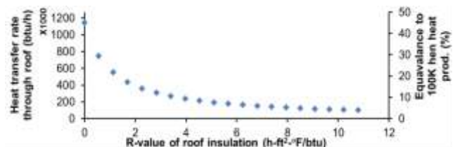
Fig 2. Heat transfer rate through the roof of the hen house with 100K hens as affected by roof insulation.
