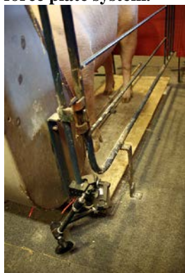
Figure 1. Sow on the embedded microcomputer-based force plate system.
