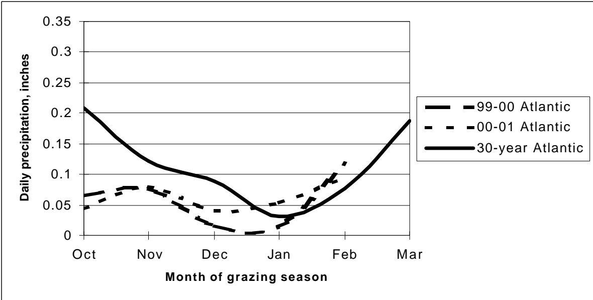
Figure 5. Atlantic daily average precipitation for 1999–2000, 2000–2001, and 30-year average.
