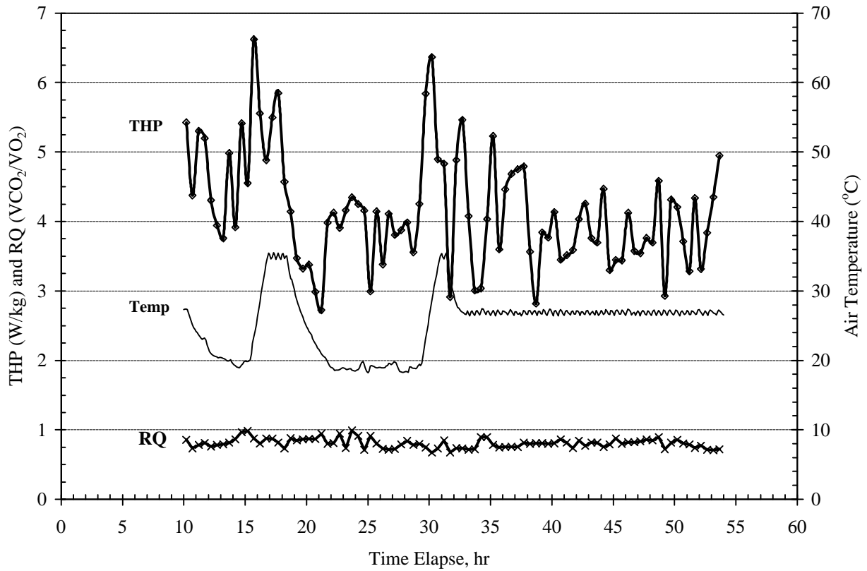
Figure 2. Dynamic total heat production (THP) and respiratory quotient (RQ) of isowean pigs exposed to 80 ± 15°F.
