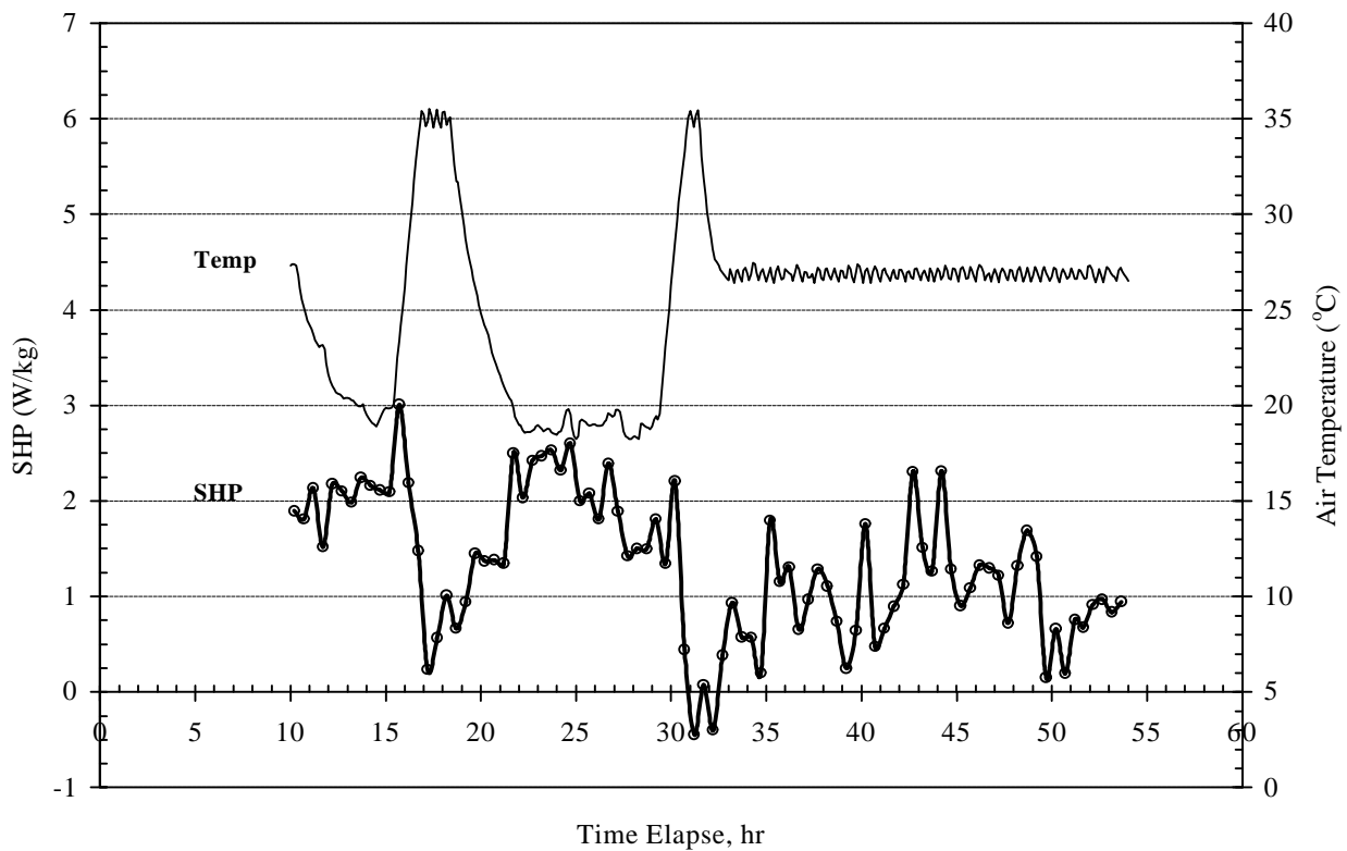
Figure 3. Dynamic sensible heat production rate (SHP) of isowean pigs exposed to 80 ± 15°F.
