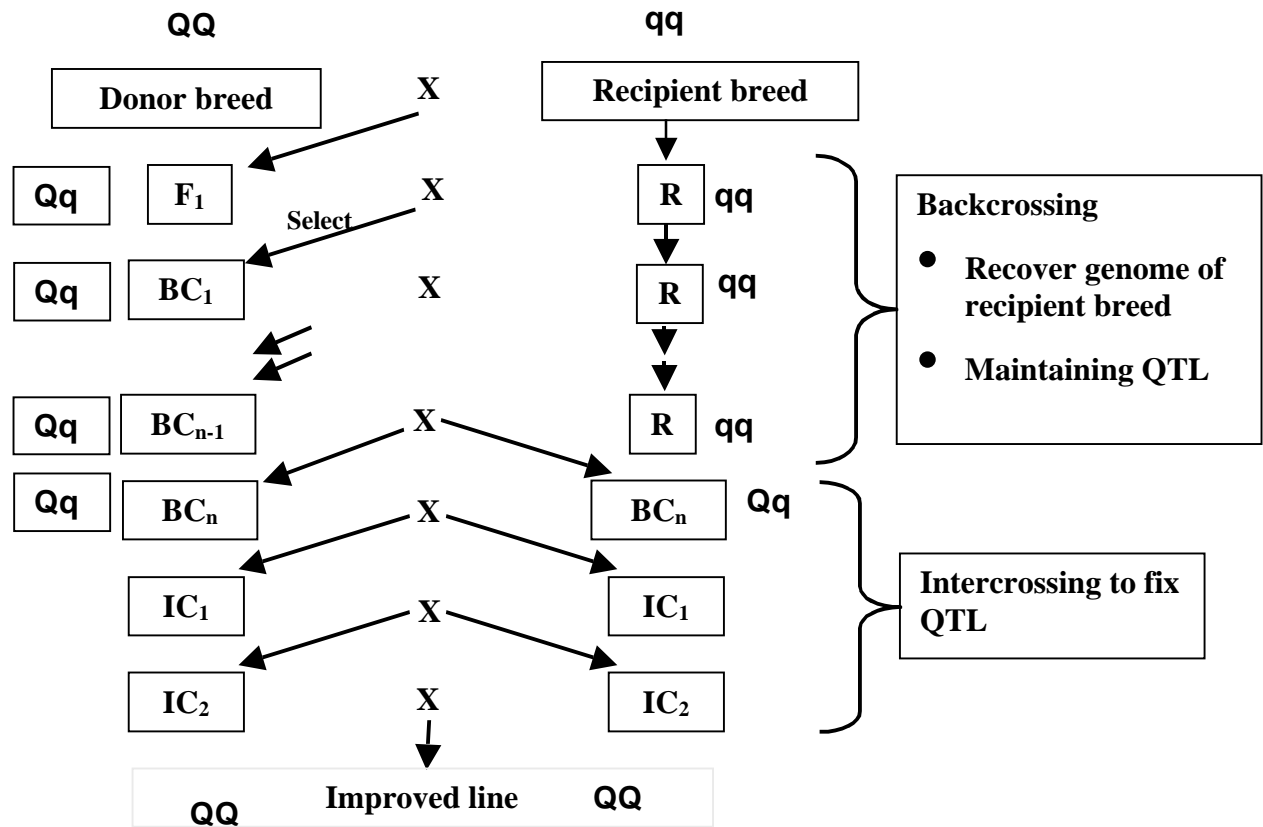
Figure 1. Two successive phases of introgressing a QTL from a donor breed (QQ genotype at QTL) into a recipient breed (qq genotype): a backcrossing phase and an interbreeding phase.
