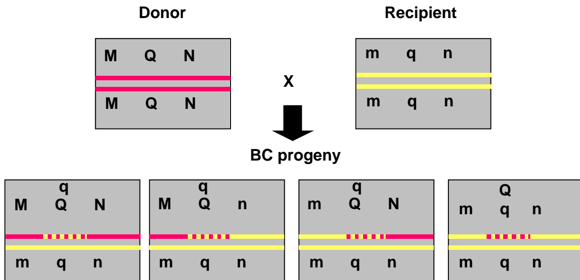
Figure 2. The inheritance of QTL and flanking markers in the backcross progeny. All backcross progeny receive one (intact) chromosome from the recipient breed and one chromosome from the BC parent. The BC chromosomes can be recombined and contain zero, one, or two marker donor alleles at flanking markers. MN chromosomes likely also contain the donor QTL allele (Q), apart from double recombination, and are the ones that are ideally selected.
