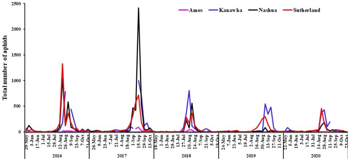
Figure 1. Seasonal population dynamics of aphids collected from suction traps located in Iowa weekly from May to October, 2016 through 2020.
