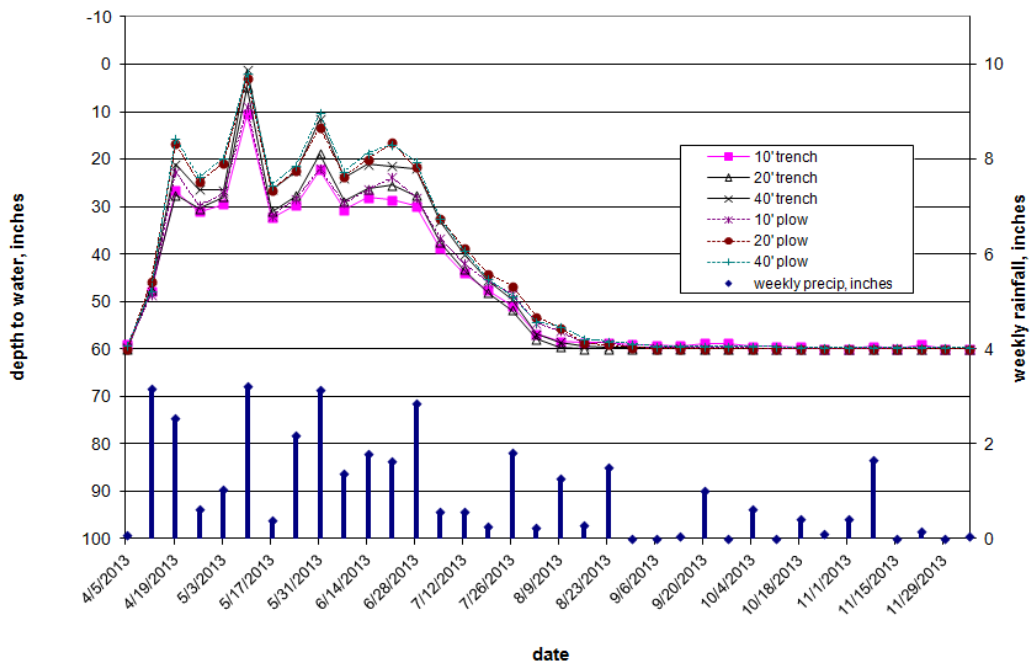
Figure 2. Water table and weekly precipitation in 2013 from two drainage installation methods at three distances.
