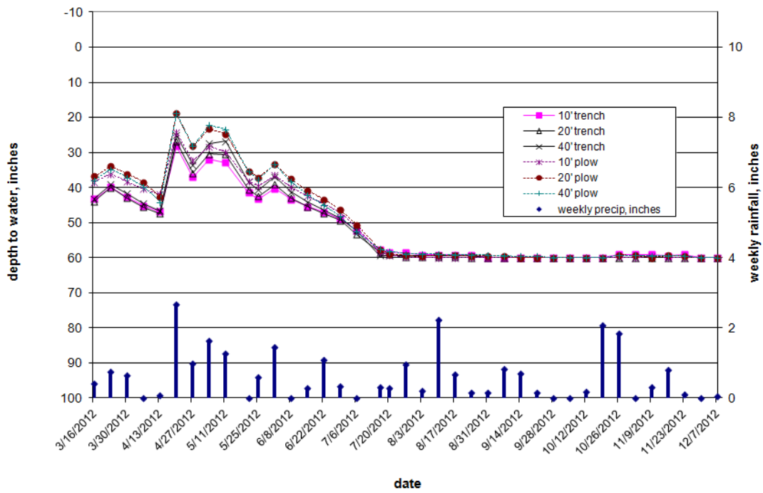
Figure 1. Water table and weekly precipitation in 2012 from two drainage installation methods at three distances.
