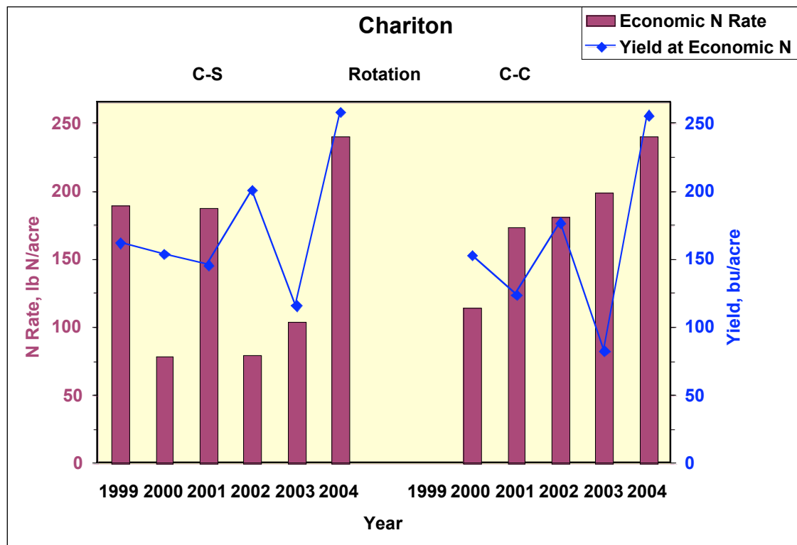
Figure 1. Corn yield and economic optimum N rate for each rotation and season, McNay Memorial Research Farm.
