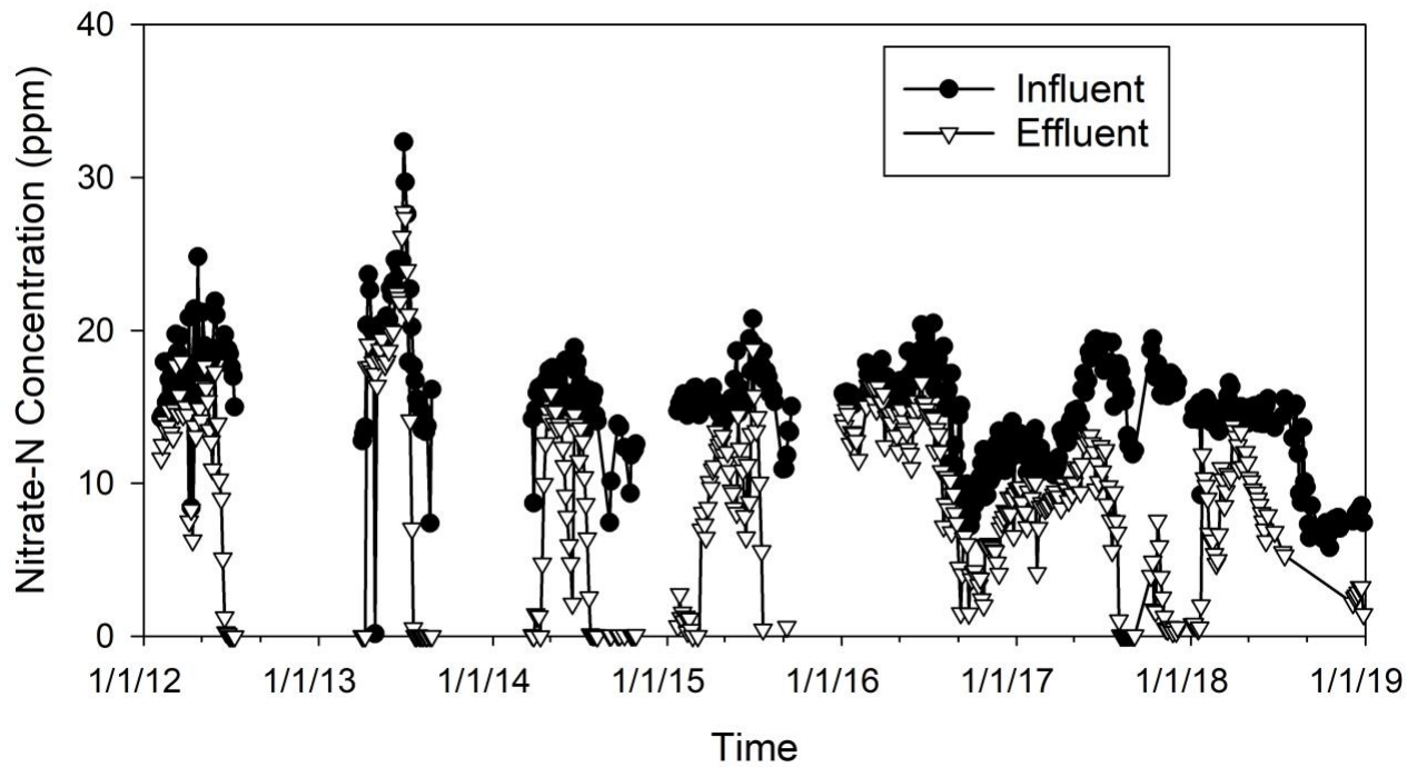
Figure 1. Nitrate-N concentrations in the bioreactor influent and effluent from 2012-2018.
