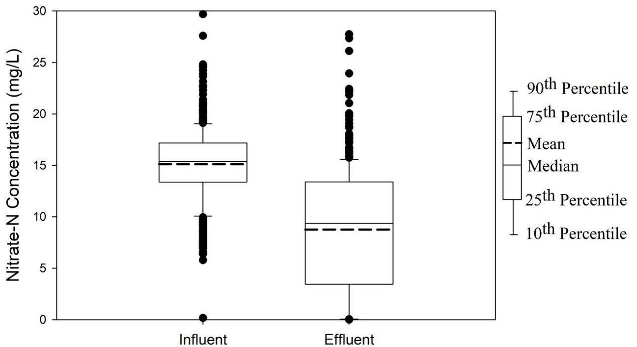
Figure 2. Box plot of nitrate-N concentrations in the influent and effluent from the bioreactor for 2012-2018.
