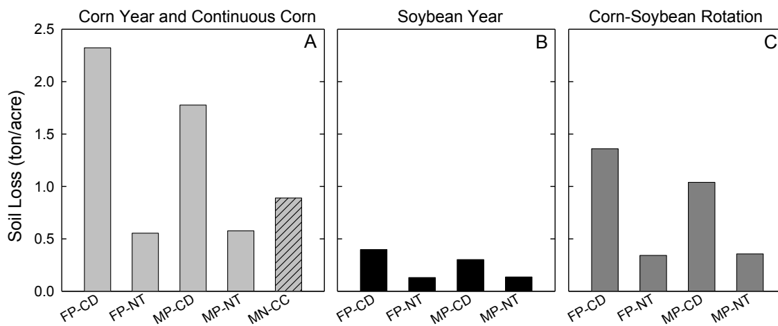
Figure 1. Amount of soil loss (6-yr averages). FP, fertilizer P; MP, manure P; CD, chisel/disk; NT, no-till; MN-CC, N-based manure for continuous corn with tillage.
