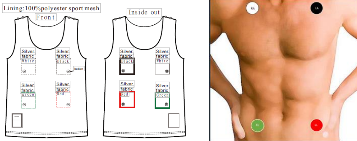
Fig. 5 Inside of lining view (Left: lining right view, Right: lining inside out view) and electrodes position
